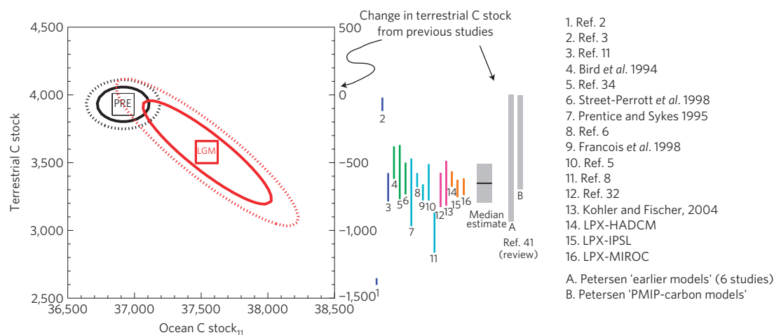
Figure 3 | Ocean and land carbon stocks inferred from carbon isotopes for the PRE and LGM. Uncertainties shown by ellipses are obtained by considering the error on each parameter entering the carbon isotope mass balance (see Supplementary Information). Solid lines are 1- \sigma uncertainty, and dotted lines are 2- \sigma uncertainty. Vertical colour bars on the right-hand side denote literature estimates of changes in global terrestrial carbon stock between the PRE and LGM. Blue (1–3), early work based on cartographic reconstructions (1) or modelling (2–3). Green (4–6), based on reconstruction of oceanic ^{13}\text{C} change, as in this study, but with older observations. Cyan (7–11), based on terrestrial-biosphere models and first-generation LGM climate models simulations from the PMIP-1 project. Magenta (12–13), based on ocean modelling. Orange (14–16), based on the LPX land-biosphere model forced by second-generation LGM climate model simulations from three models of the PMIP-2 program (those that had archived the necessary variables used to run LPX; see Supplementary Information). The grey bar is the median of estimates 1–16 plus or minus one median absolute deviation, excluding proven unrealistic estimates 1 and 2. The grey bars labelled A and B are the range of various published global terrestrial carbon stock values during the LGM from the review in ref. 41.
