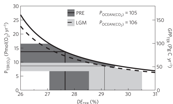
Figure 2 | Relationship defining terrestrial photosynthesis ( GPP_{\text{TER}} ) as a function of the ^{18}\text{O} isotopic enrichment of land oxygen fluxes, or land Dole effect, DE_{\text{TER}} . Simulations of DE_{\text{TER}} for the PRE (dark grey) and LGM (light grey), together with measurements of ^{18}\text{O} in atmospheric oxygen from ice cores, allow GPP_{\text{TER}} during the LGM to be constrained. P_{\text{TER}(\text{O}_2)} is the global flux of oxygen (left-hand axis) emitted by terrestrial photosynthesis, about two times GPP_{\text{TER}} . The lines depend on ocean productivity for the PRE (solid) and LGM (dashed). Shaded grey uncertainties are calculated with Monte Carlo analysis of ocean and land parameters (see Supplementary Information).
